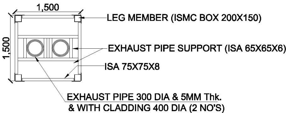
SECTION X-X
