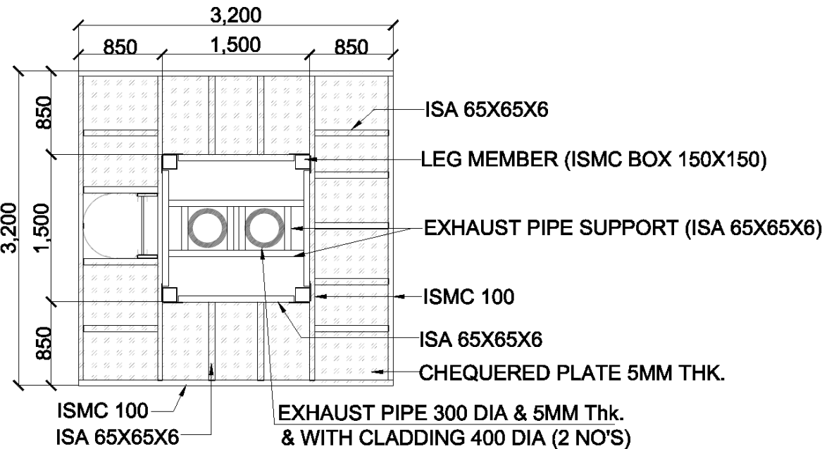
PLATFORM DETAILS
